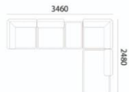
HW01A-1 + HW01B-1 + HW01A-1 + HW01D-1 + HW01F-1 3460*2480*700MM 136.2*97.6*27.6"
